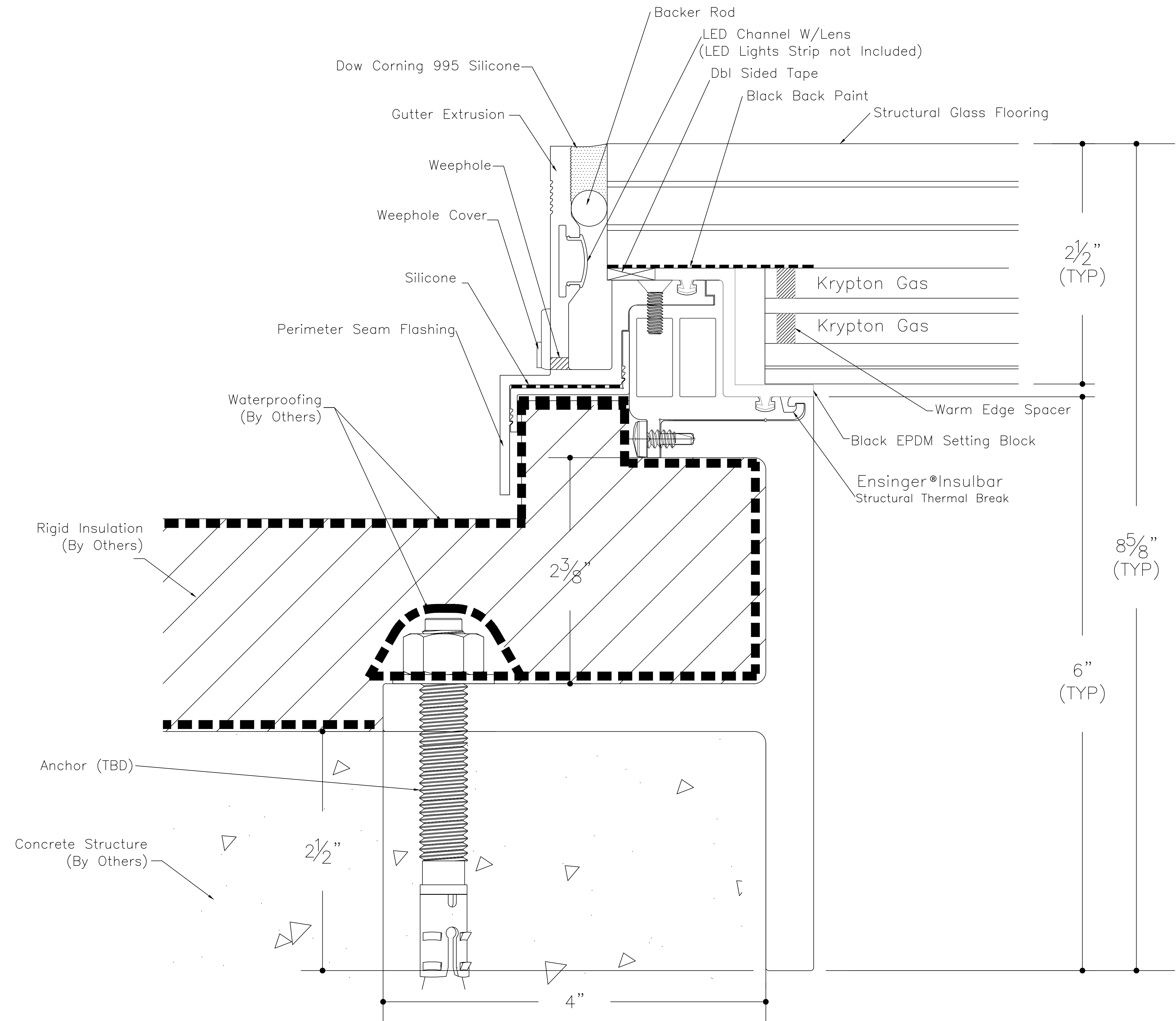
① SkyFloor® Series 2000 Recessed perimeter with Double Spacer
