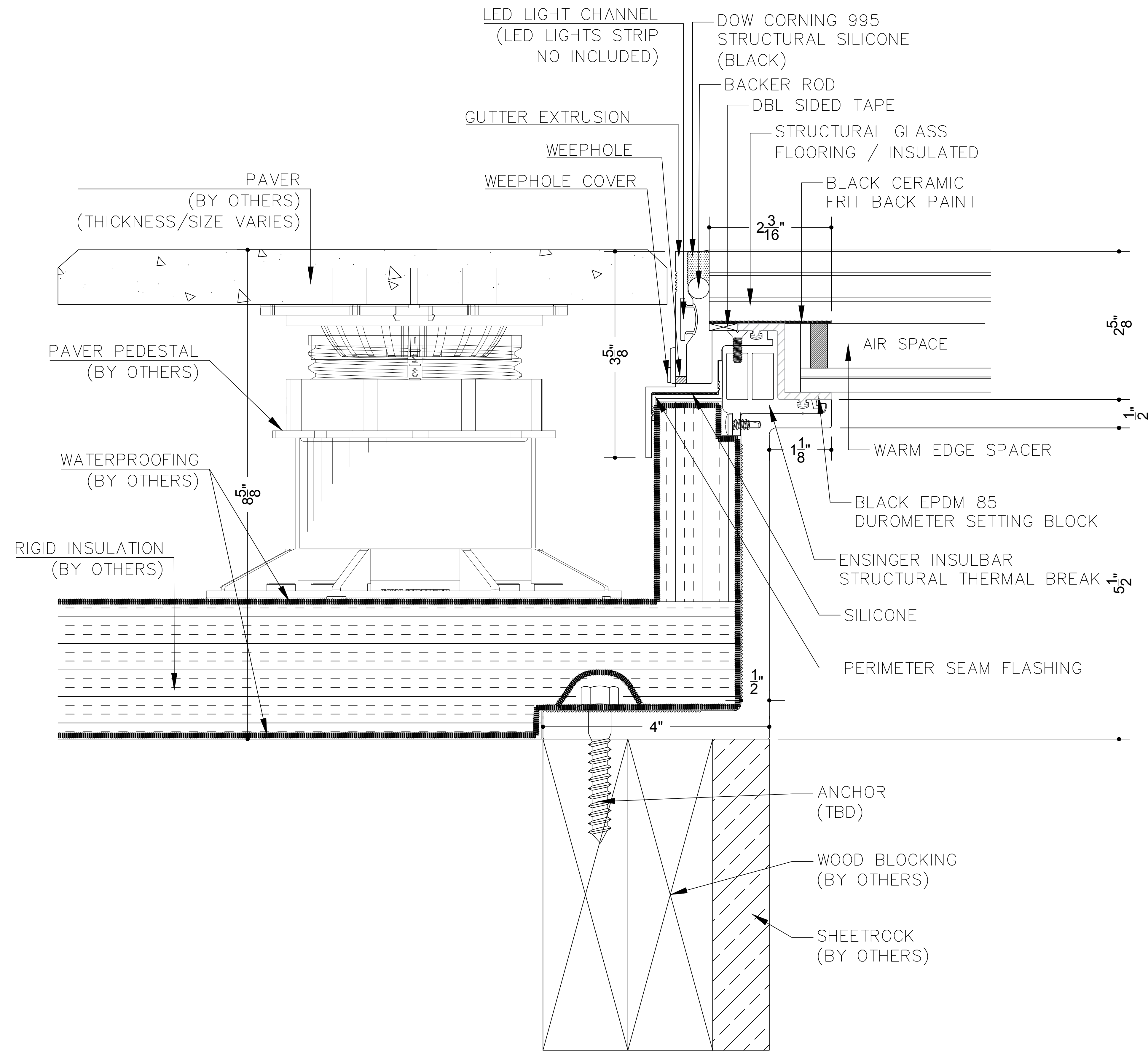
1 DETAIL - THERMALLY BROKEN PEDESTAL PERIMETER WITH WOOD Scale: 1'-0"=1'-0"
