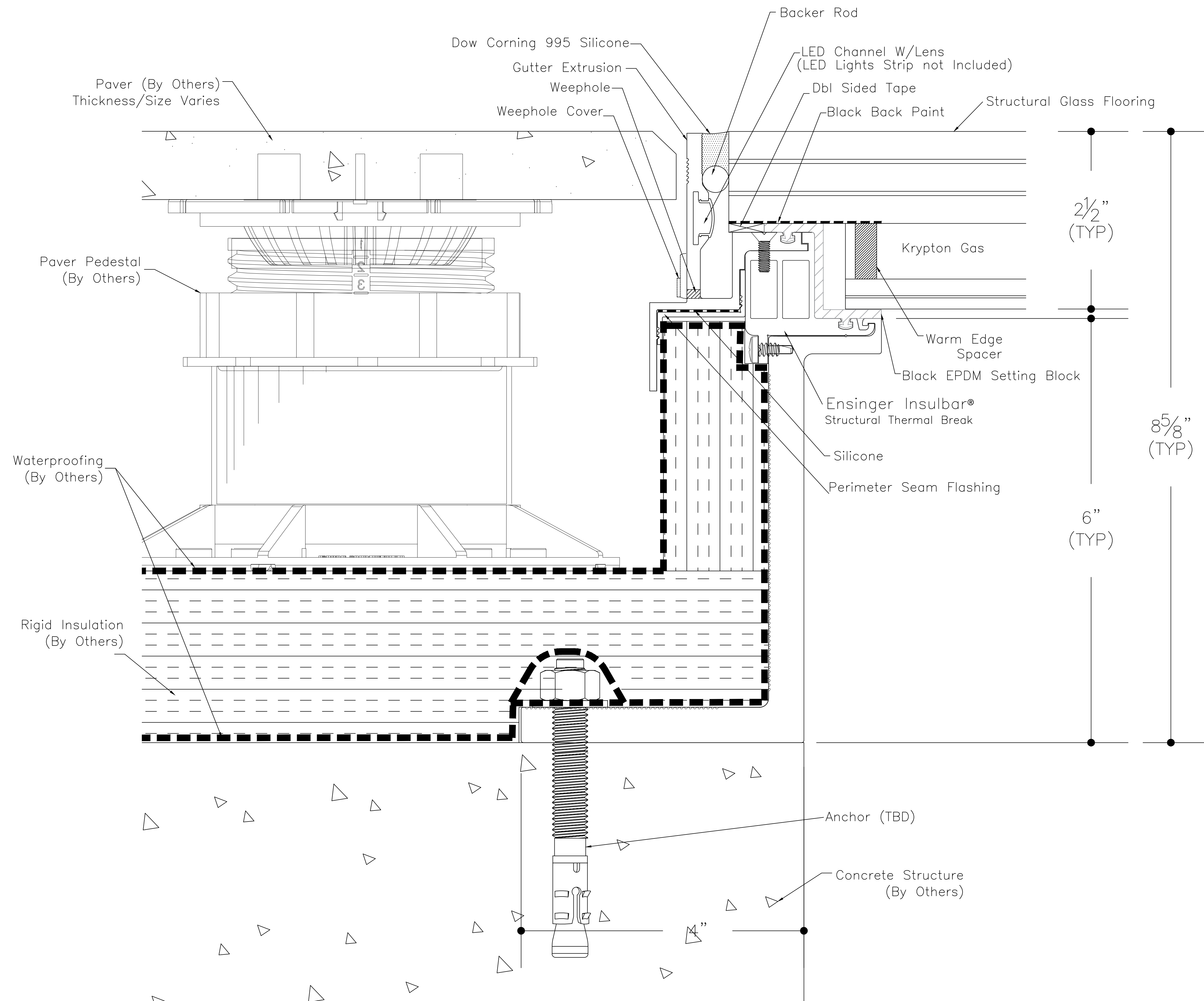
① SkyFloor® Series 2000 Pedestal perimeter with Single Spacer with concrete
