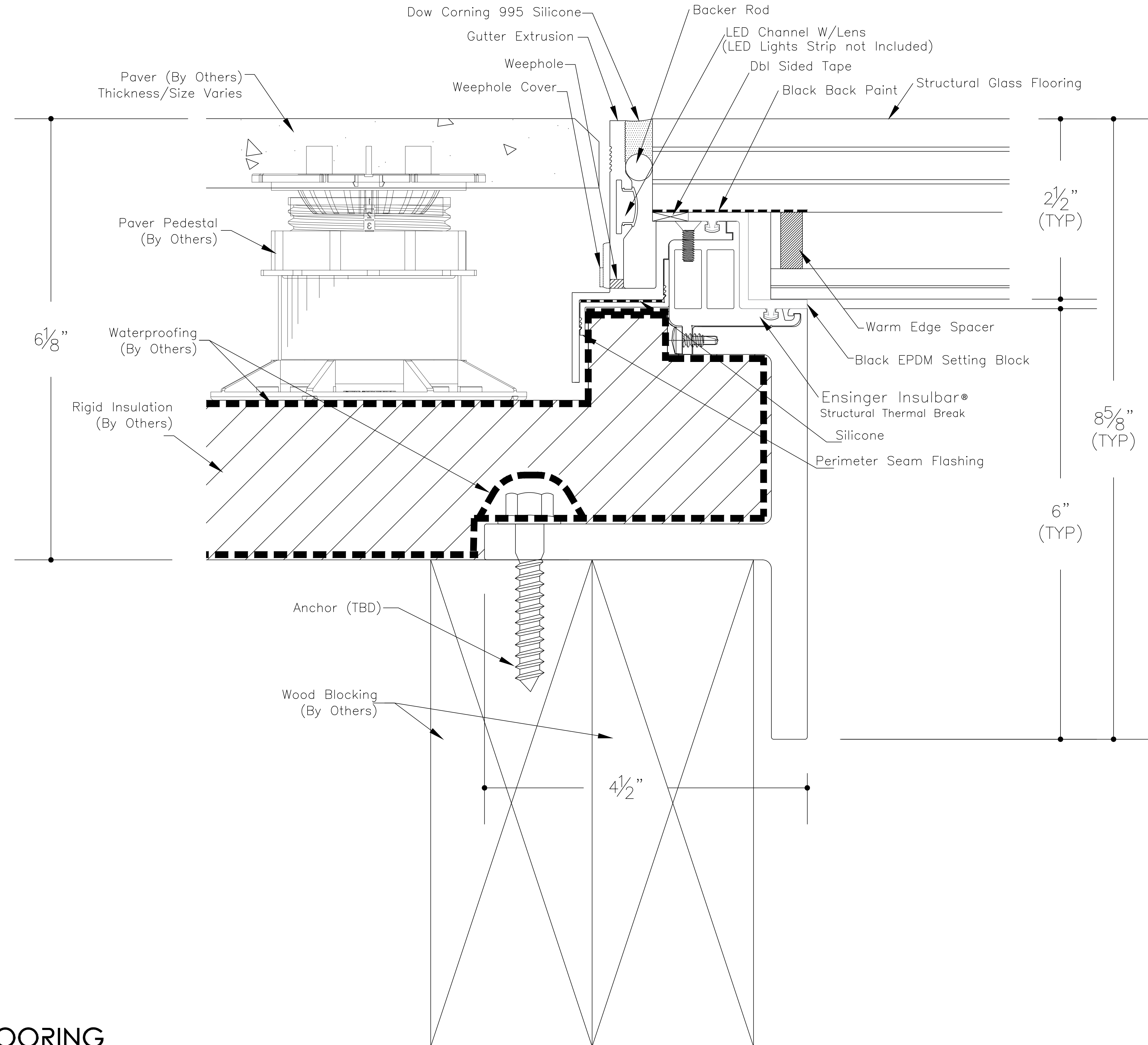
① SkyFloor® Series 2000 Recessed Perimeter With Single Spacer With Wood
