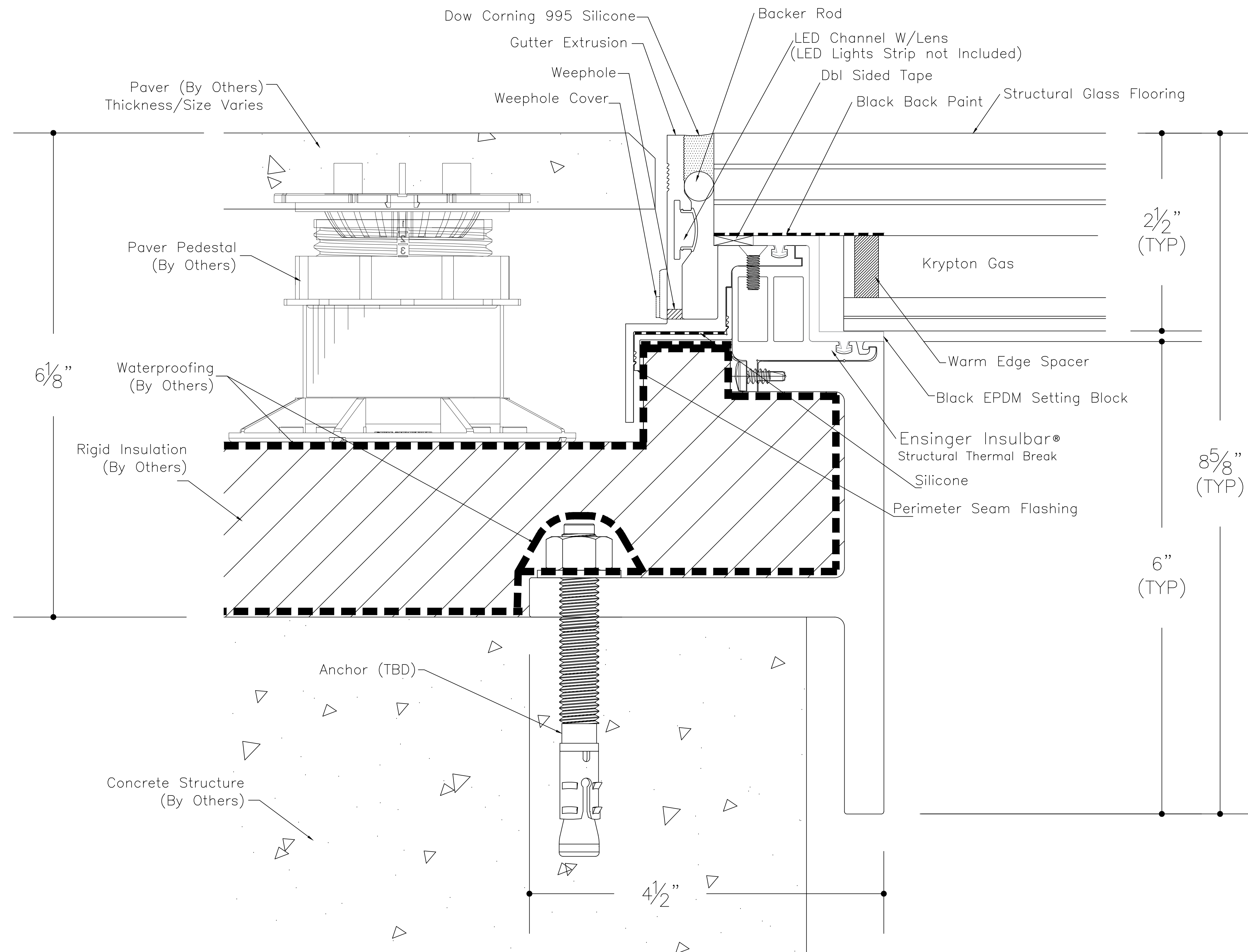
① SkyFloor® Series 2000 Recessed perimeter with Single Spacer With Concrete
