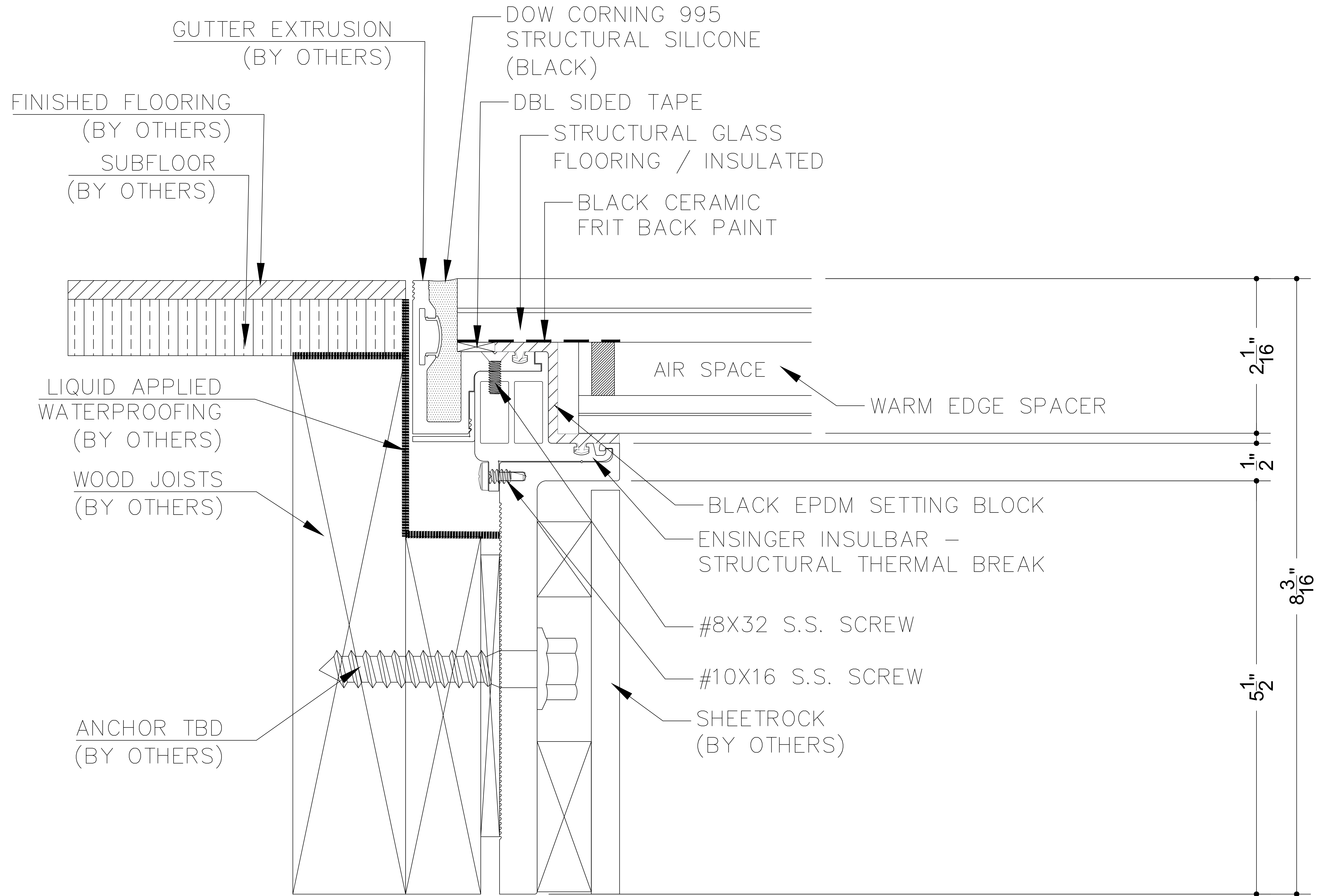
1 DETAIL - MODIFIED THERMALLY BROKEN NON-WALKABLE SERIES 2.0 PEDESTAL PERIMETER Scale: 1'-0"=1'-0"
