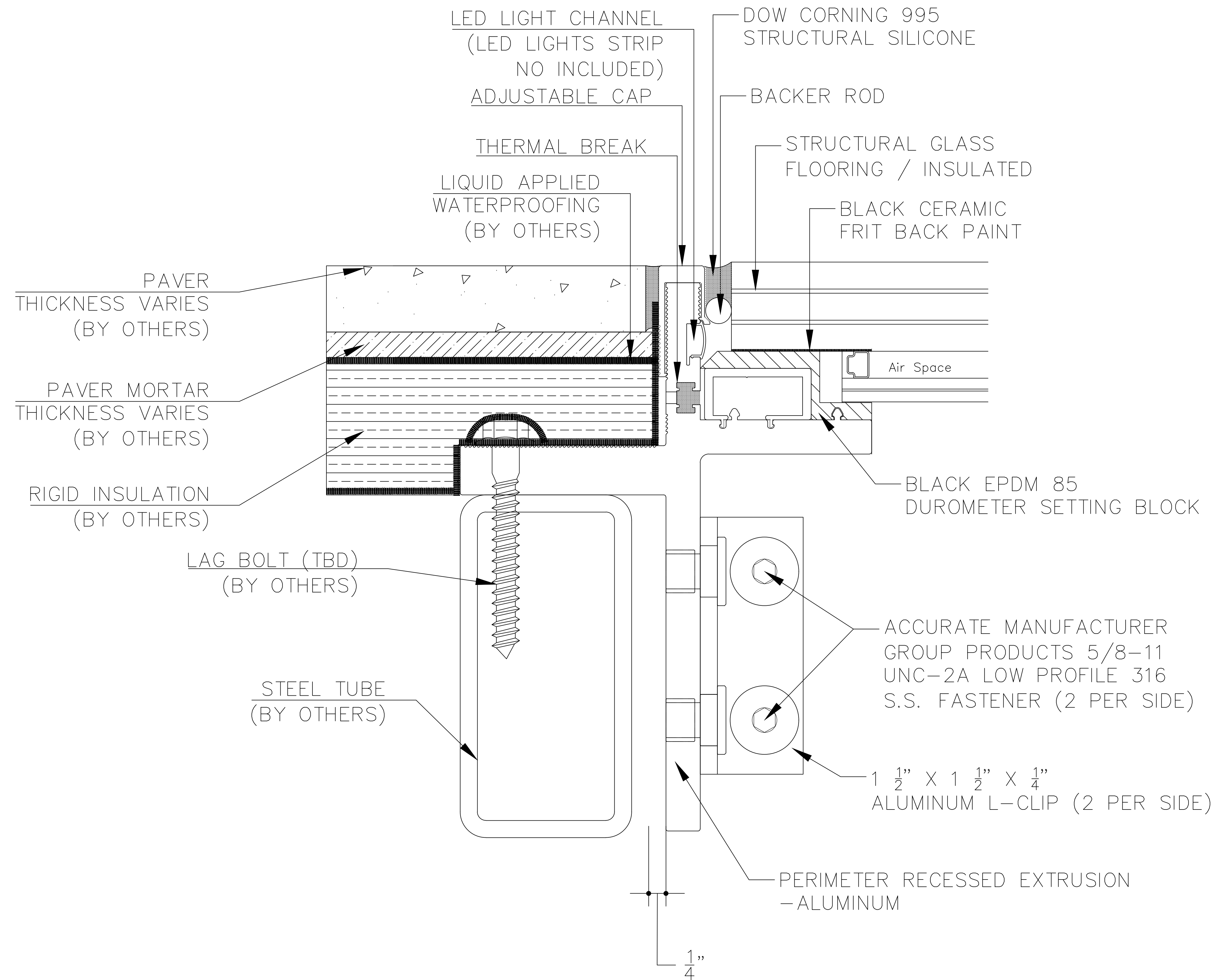
SkyFloor® Series 1000 Thermally Broken Recessed Perimeter with Steel Tube
