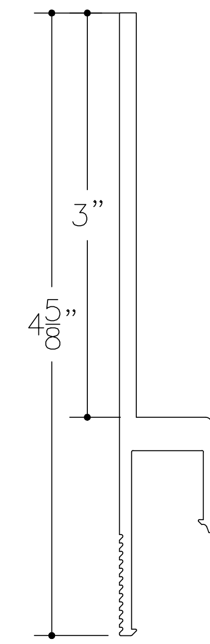
Custom 3" Vertical Adjustable Top Cap (Option A)
