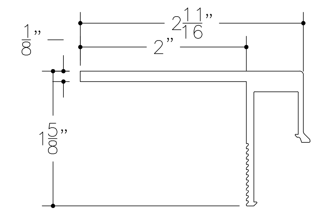
Custom 2" Horizontal Adjustable Top Cap (Option C)
