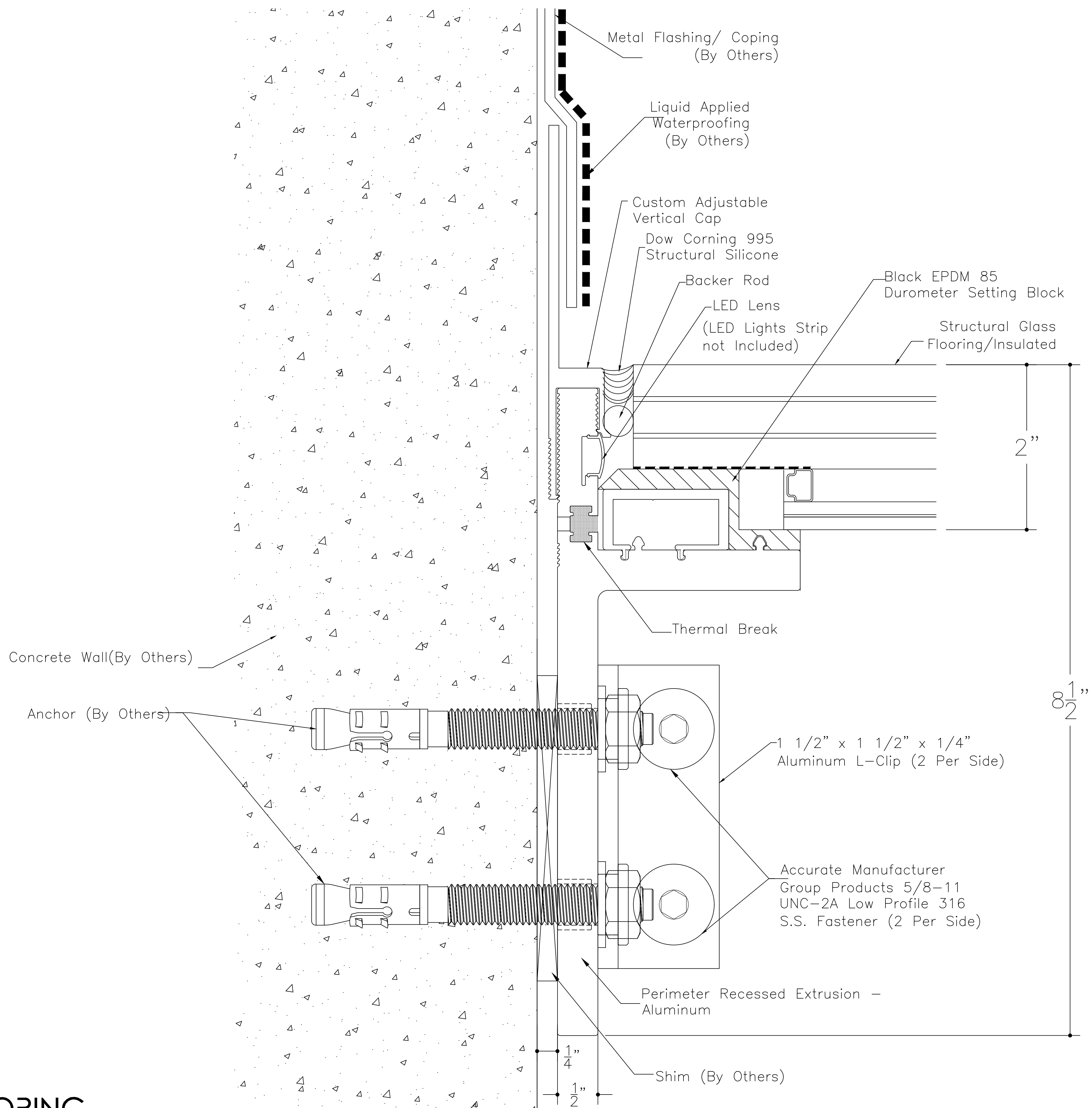
SkyFloor® Series 1000 Exterior Recessed Paver Detail with Concrete Wall- Rear Flange Off
