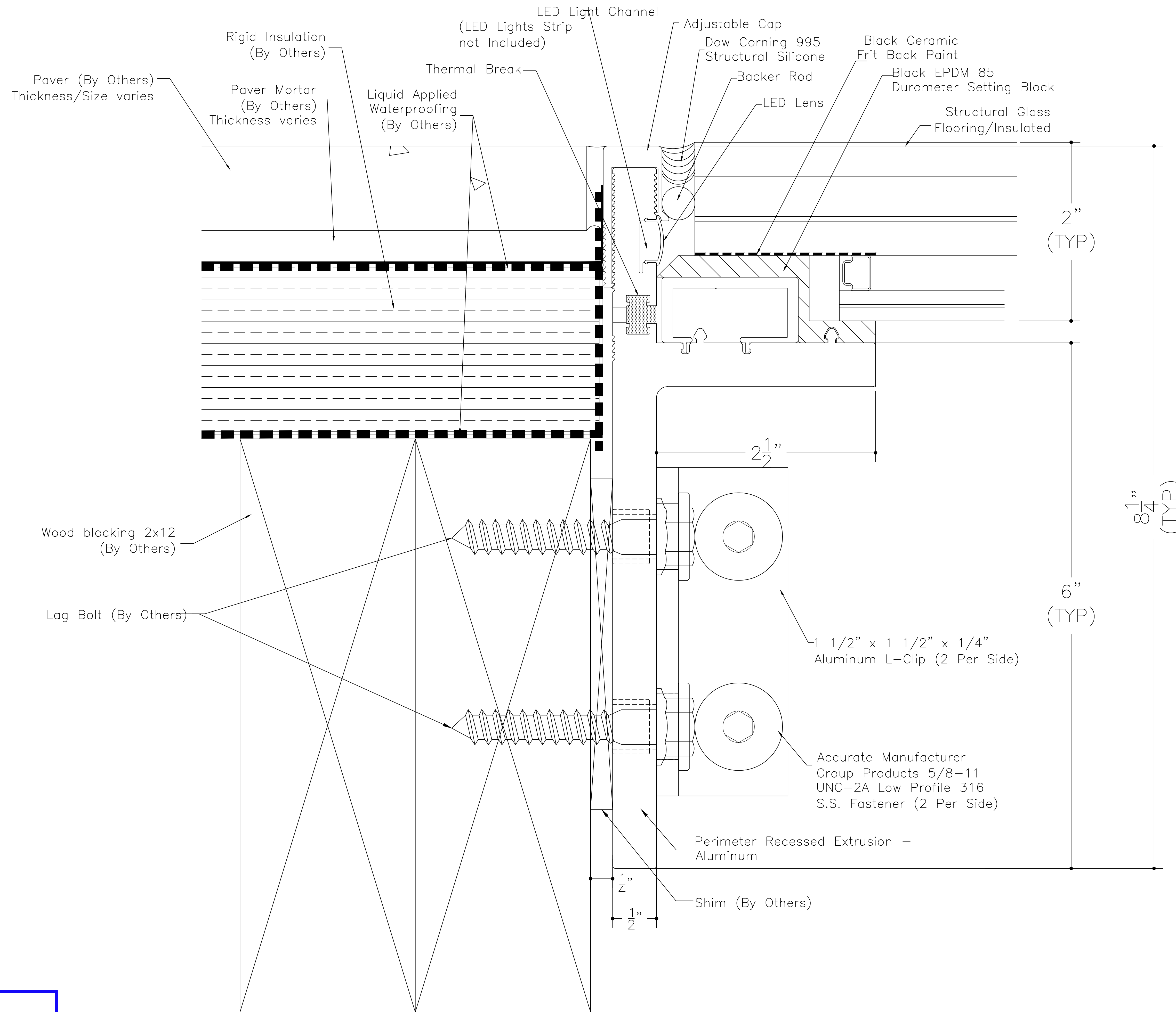
SkyFloor® Series 1000 Exterior Recessed Paver Detail with Wood Block- Rear Flange Off
