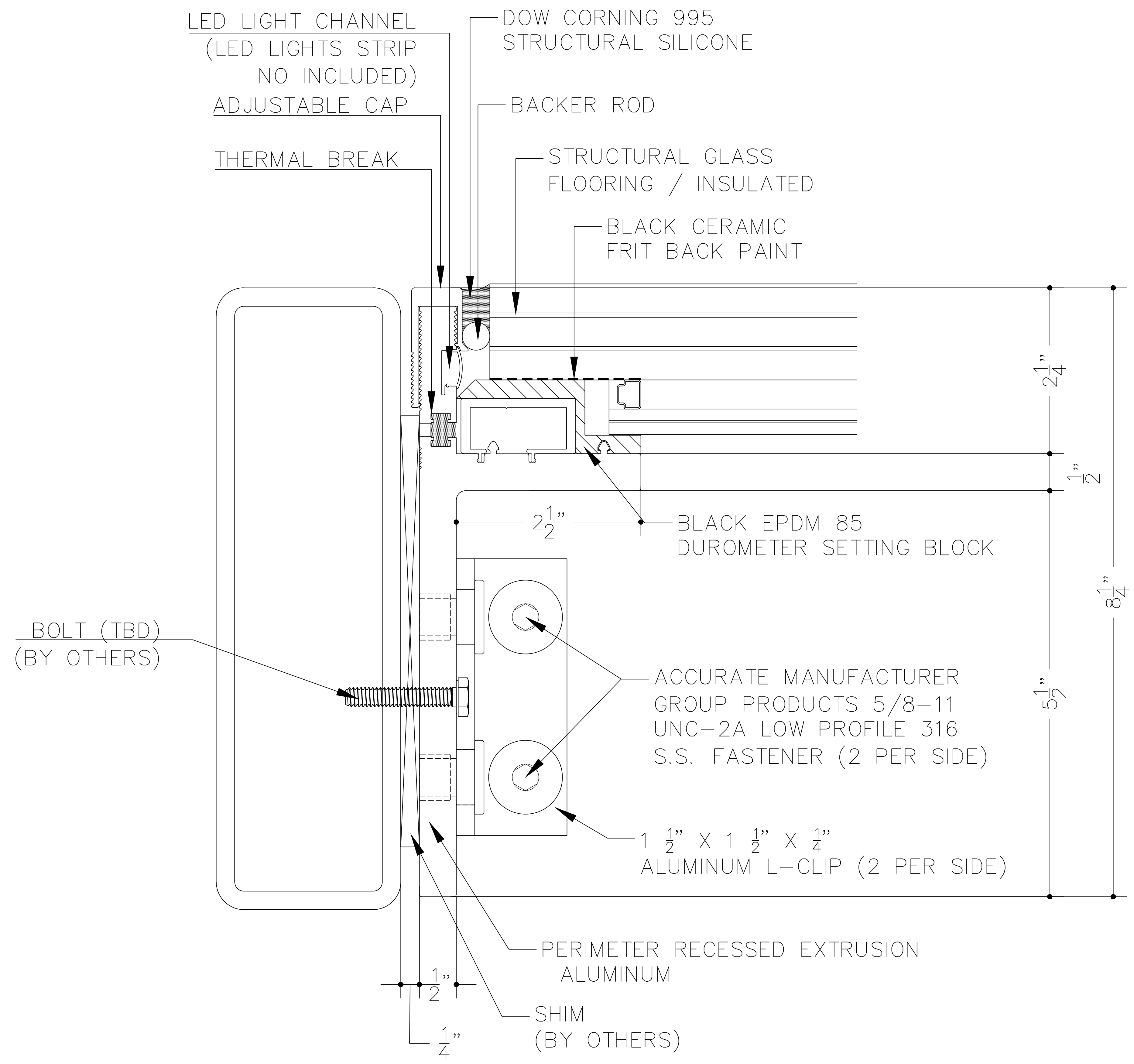
SkyFloor® Series 10000 Exterior Walkable Skylight Recessed Details - Rear Flange Off
