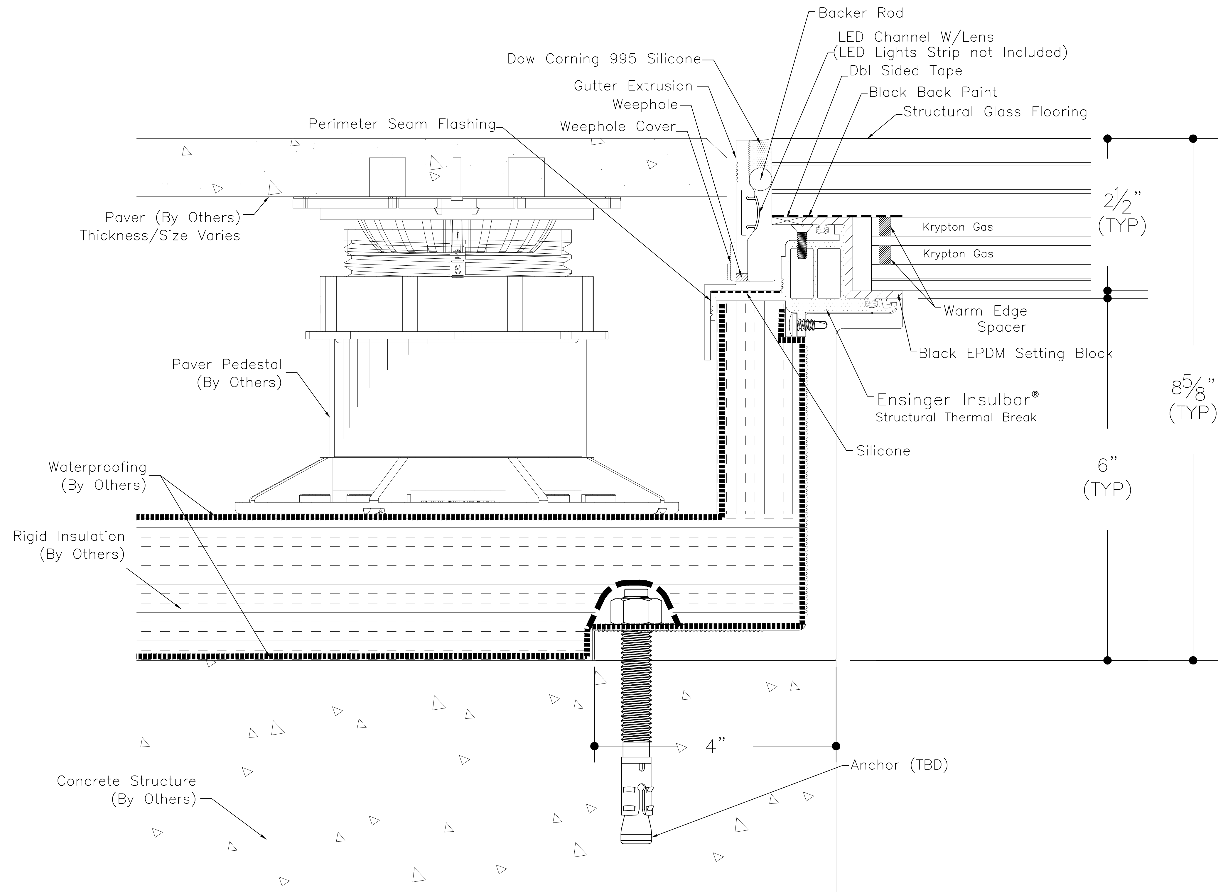
① SkyFloor® Series 2000 Pedestal perimeter with Double Spacer
