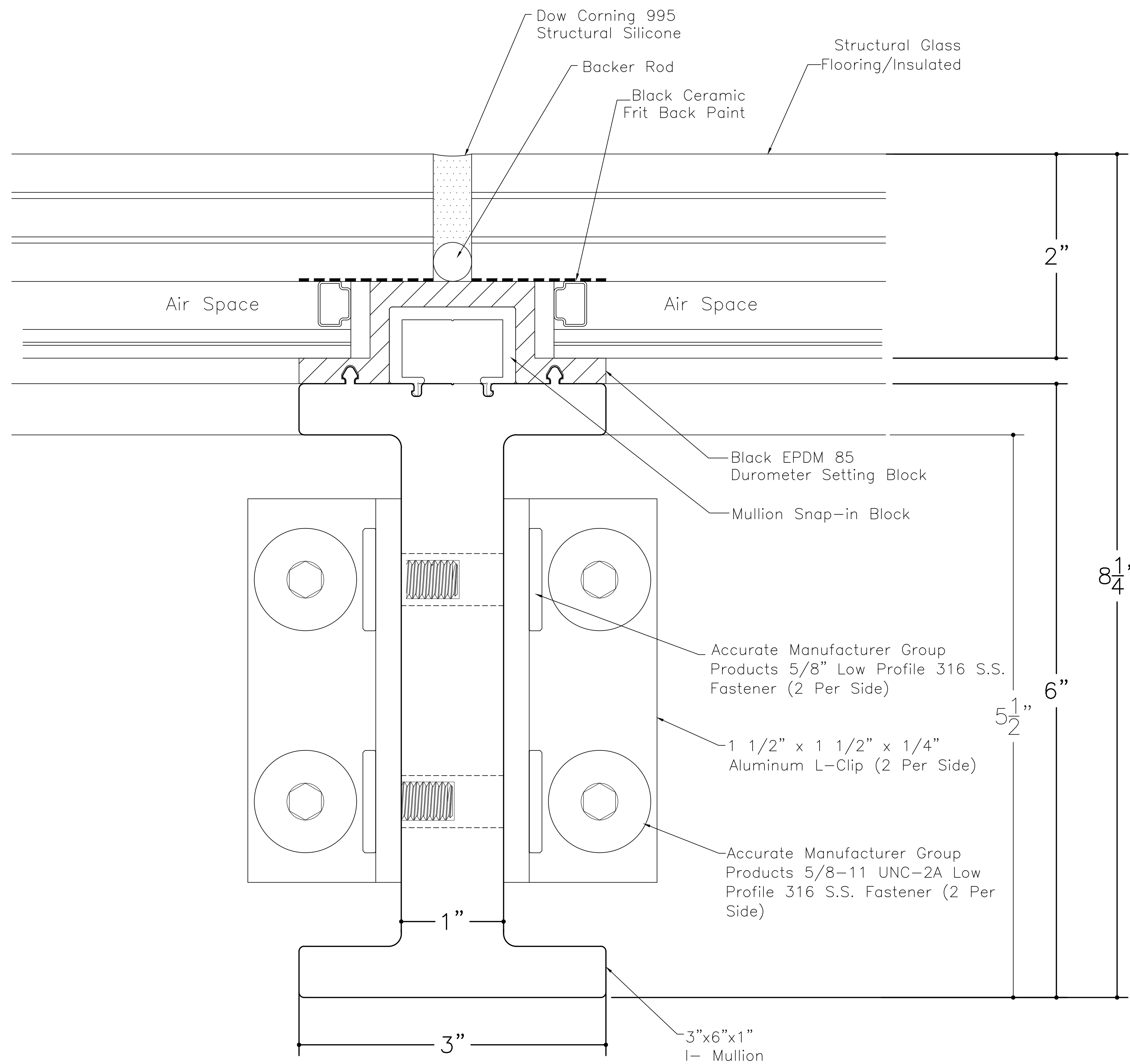
SkyFloor® Series 1000 Thermal I -Rafter
