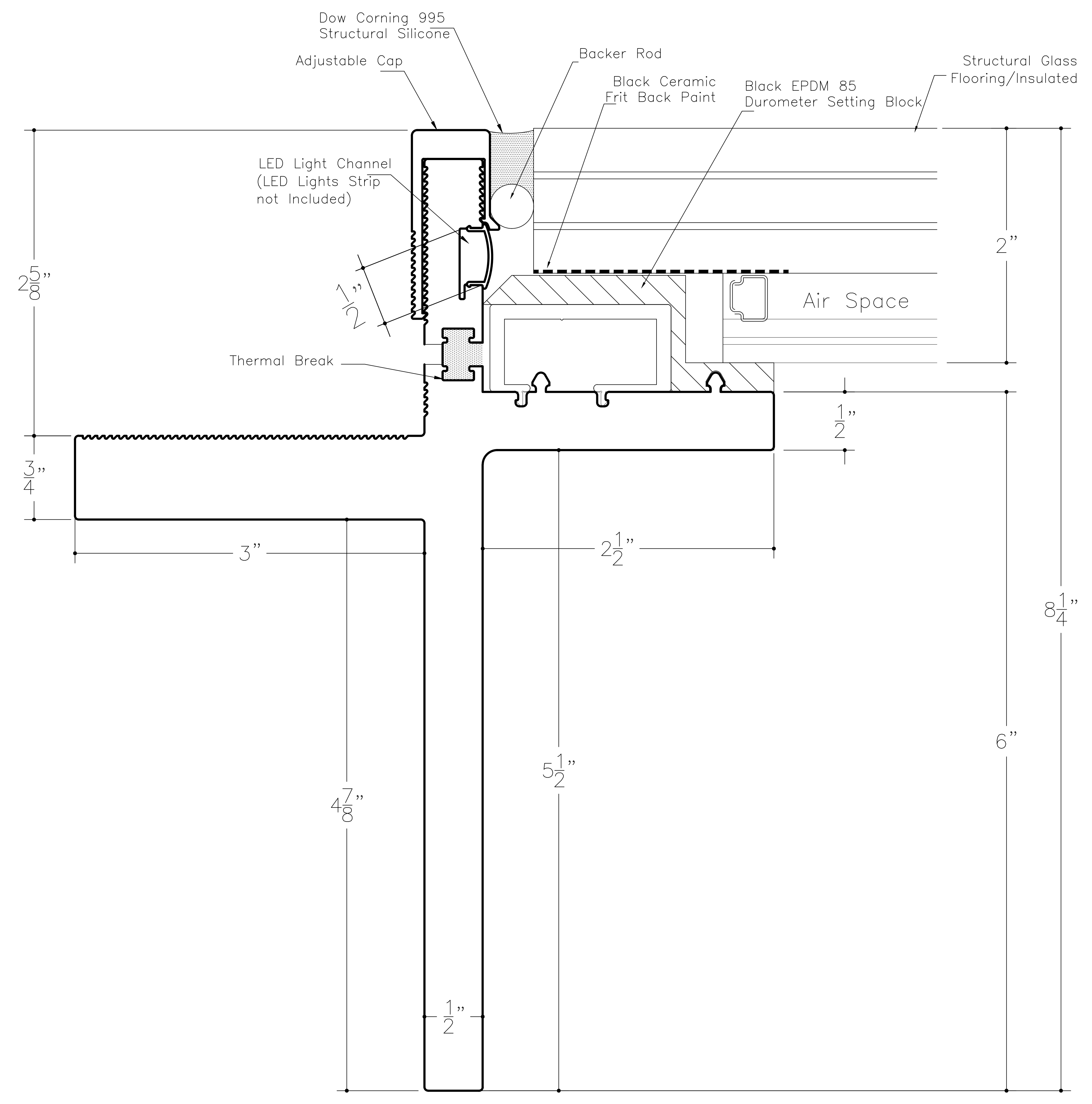
SkyFloor® Series 1000 Recessed Perimeter
