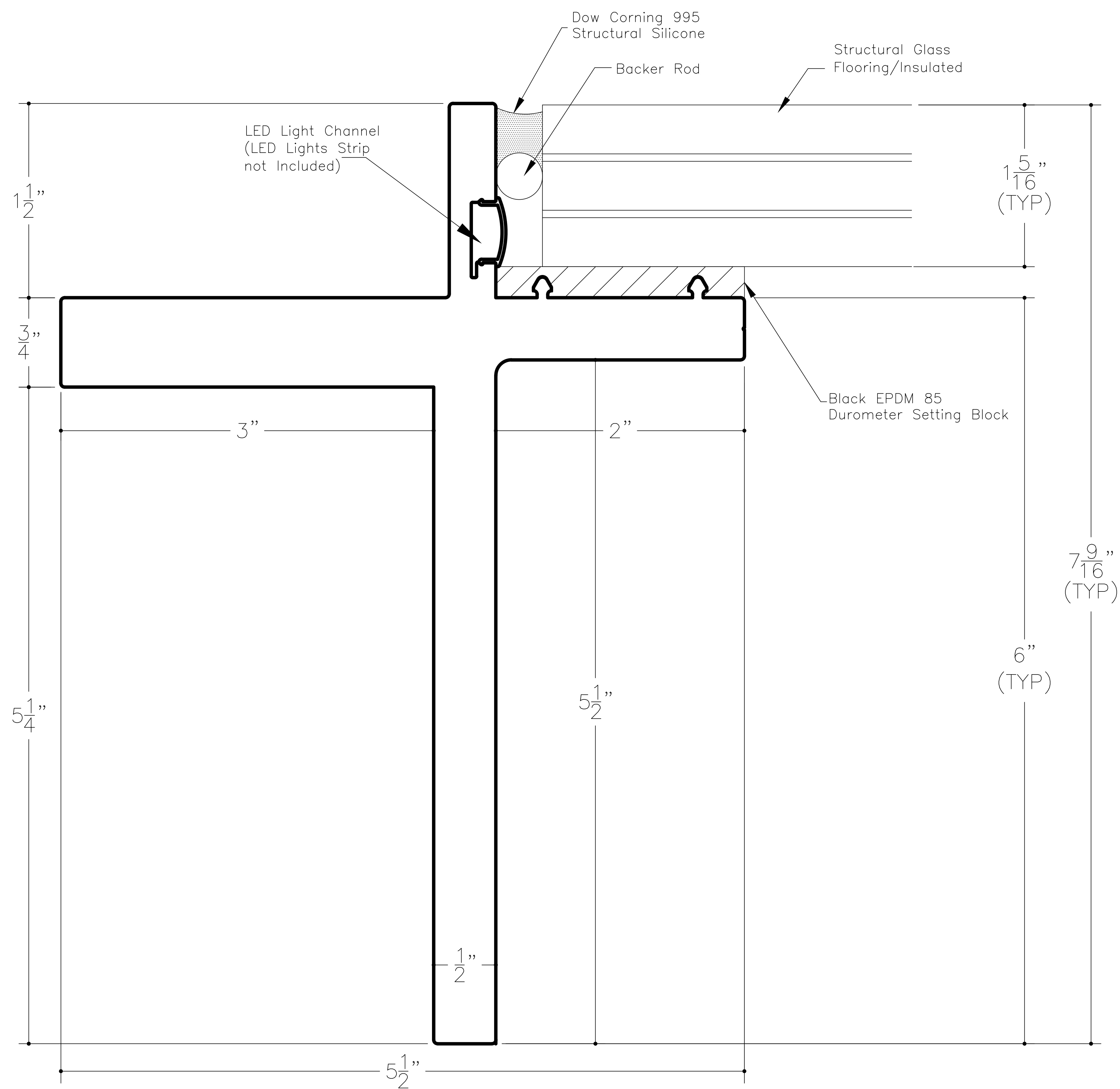
SkyFloor® Series 1000 Non Thermal Perimeter
