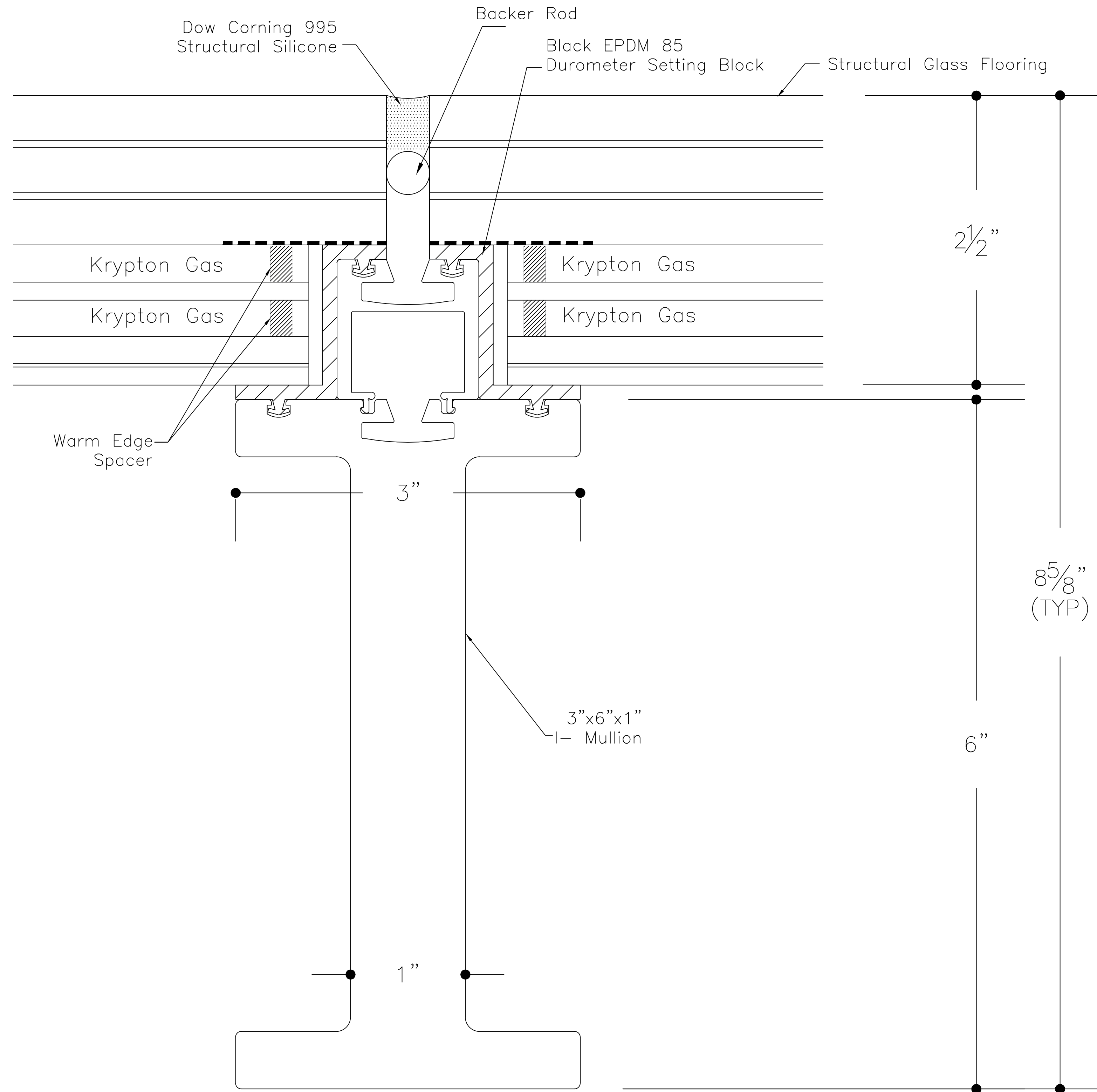
① SkyFloor® Series 2000 I Mullion with Double Warm Edge Spacer
