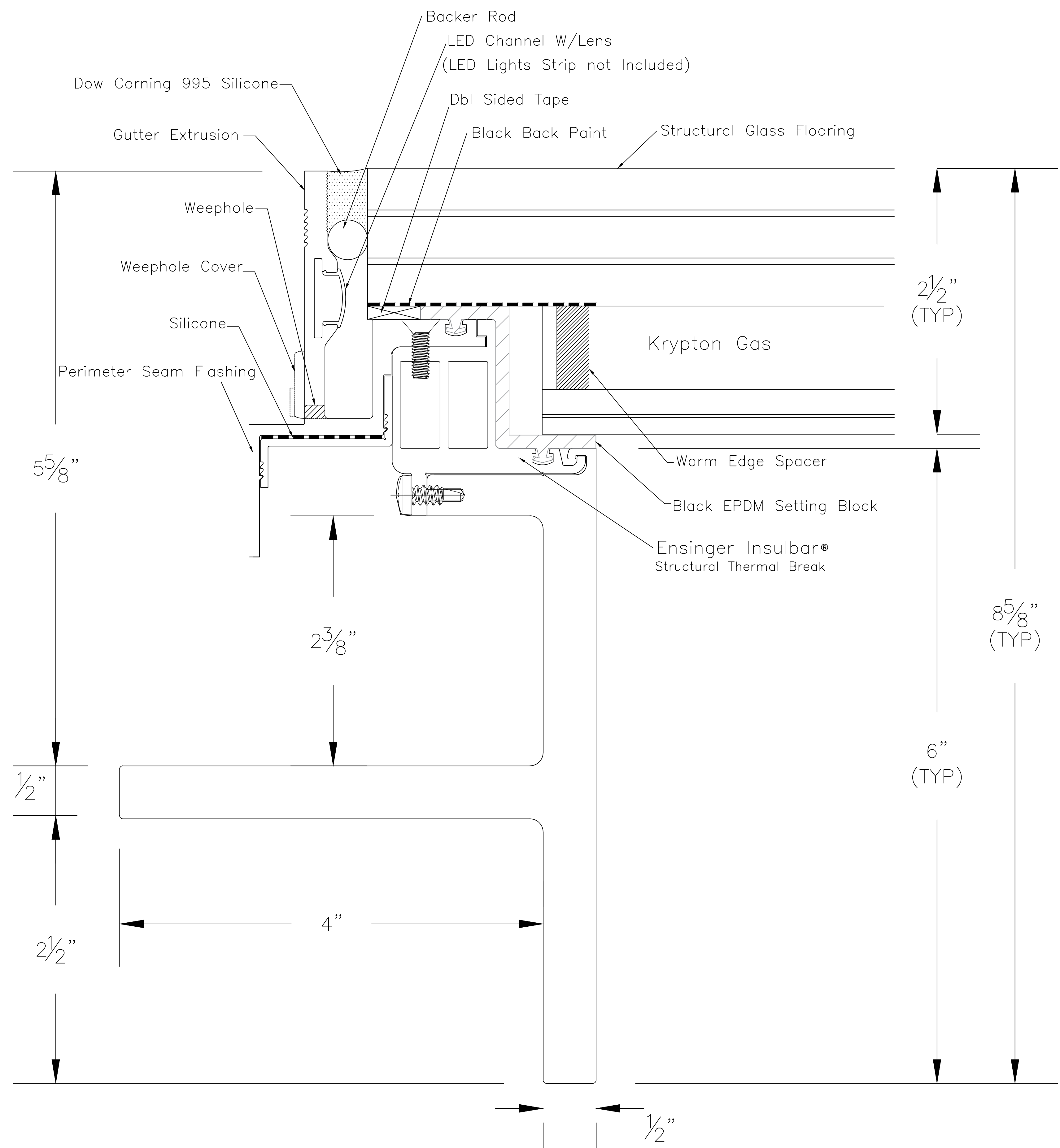
SkyFloor® Series 2000 Recessed Perimeter with Single Spacer
