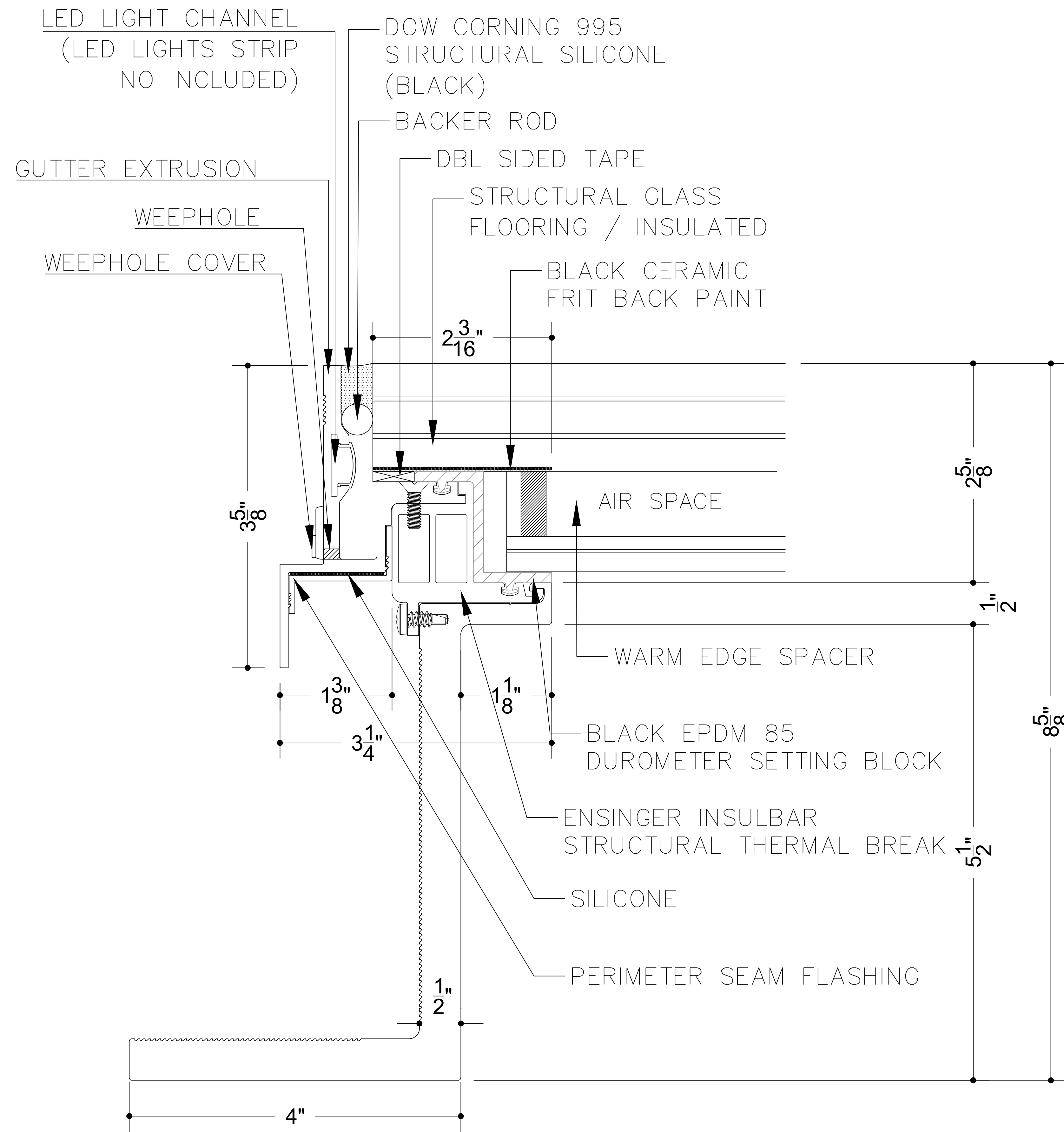
1 DETAIL - THERMALLY BROKEN PEDESTAL PERIMETER Scale: 1'-0"=1'-0"
