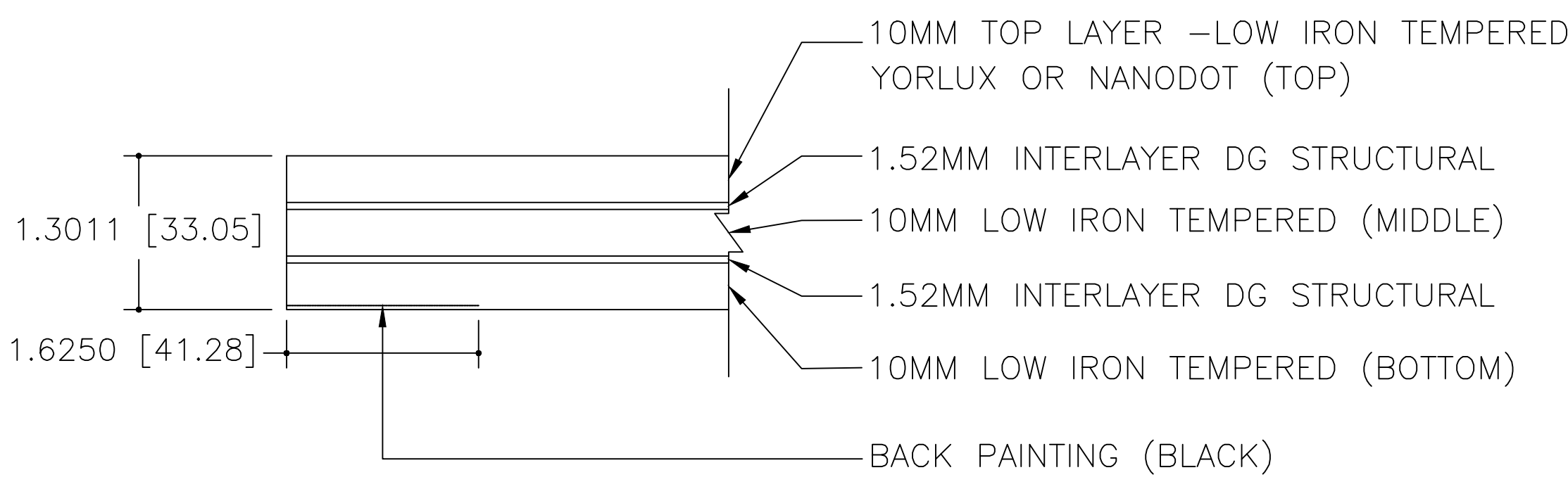
DETAIL - GLASS ASSEMBLY
