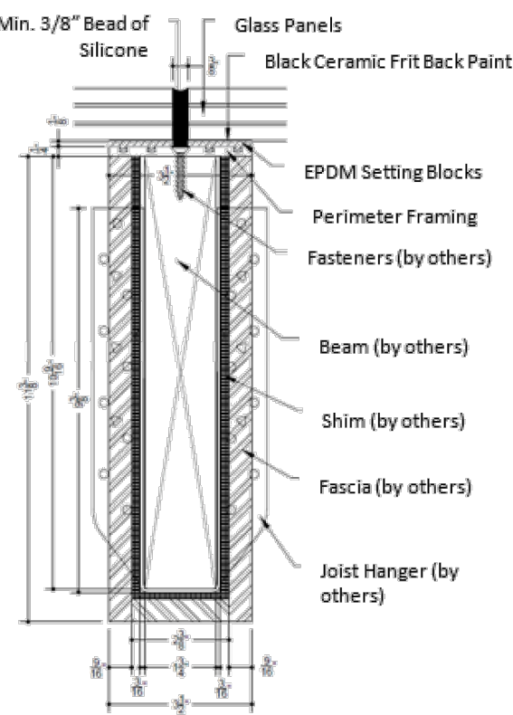
FIGURE 2 - PERIMETER DETAIL BETWEEN ADJACENT GLASS PANELS (except for silicone, dimensions are shown for illustrative purposes only)
