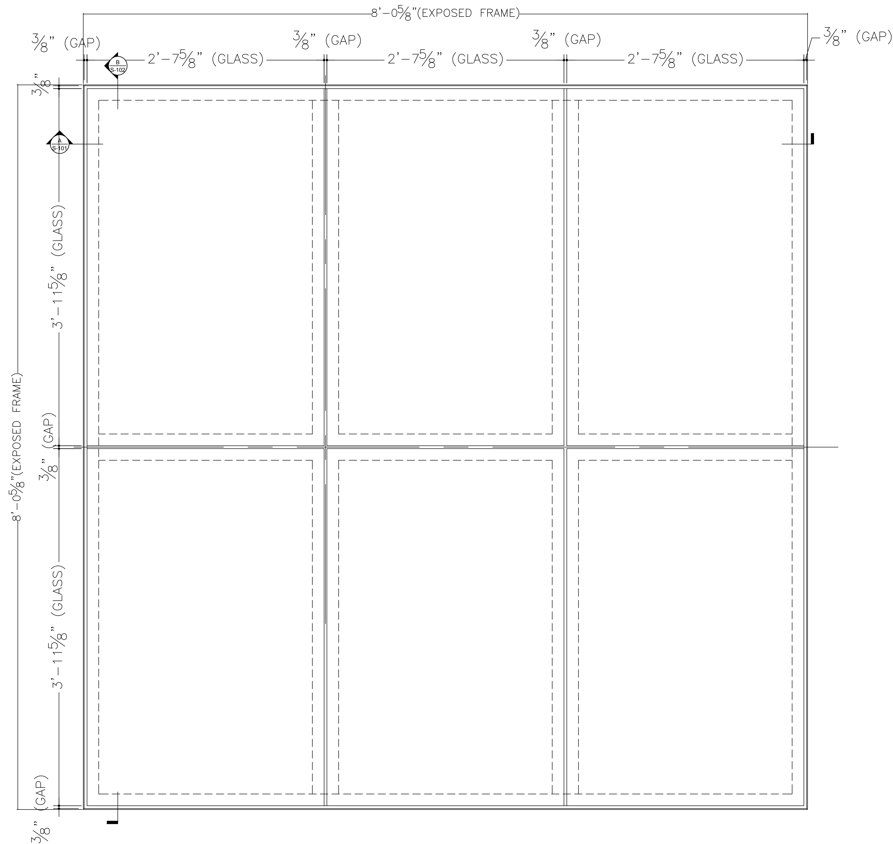
PLAN VIEW - MULTI-PANEL UNIT A
