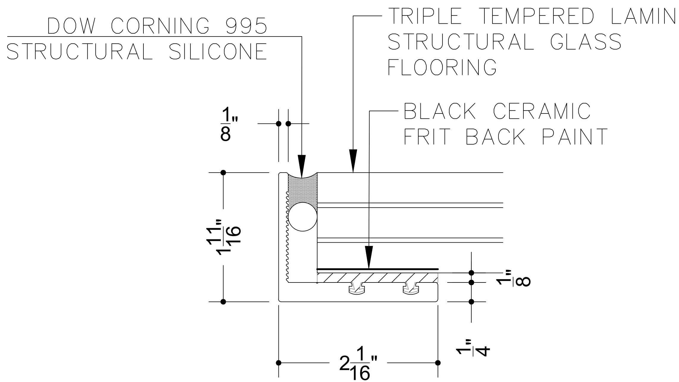
DETAIL - SKYFLOOR® MODULAR GLASS DECK PERIMETER
