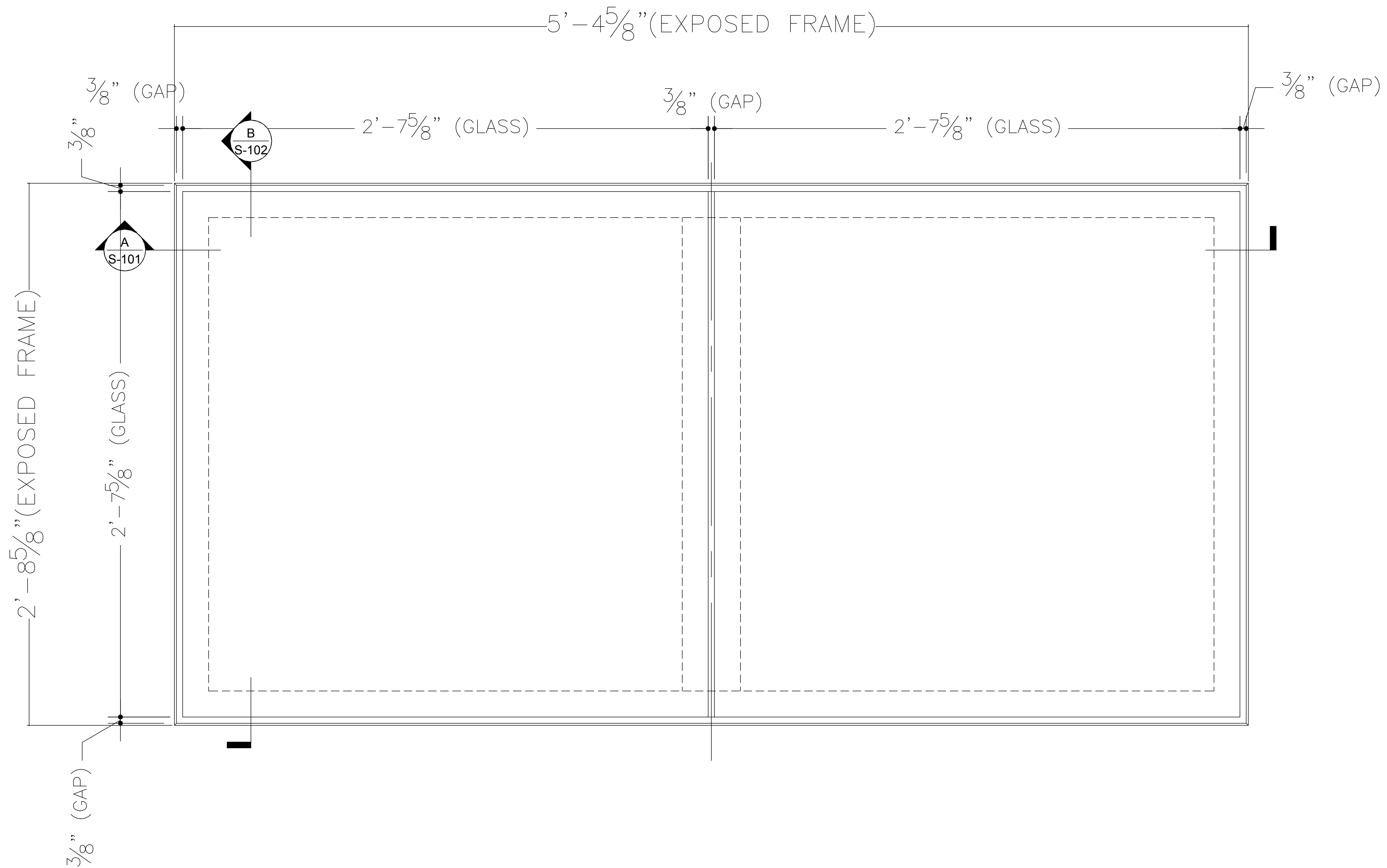
PLAN VIEW - MULTI-PANEL UNIT A
