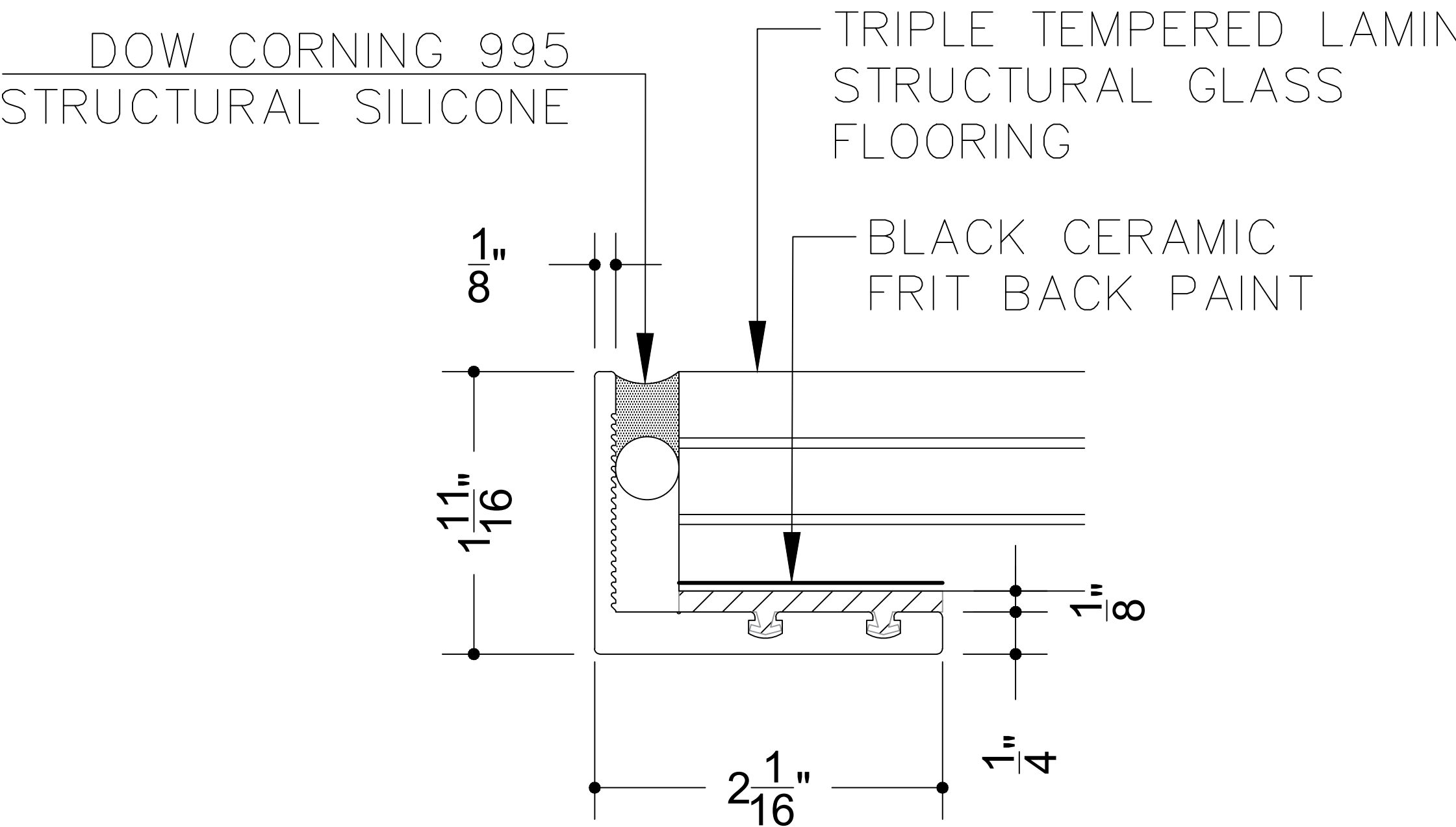
DETAIL - SKYFLOOR® MODULAR GLASS DECK PERIMETER
