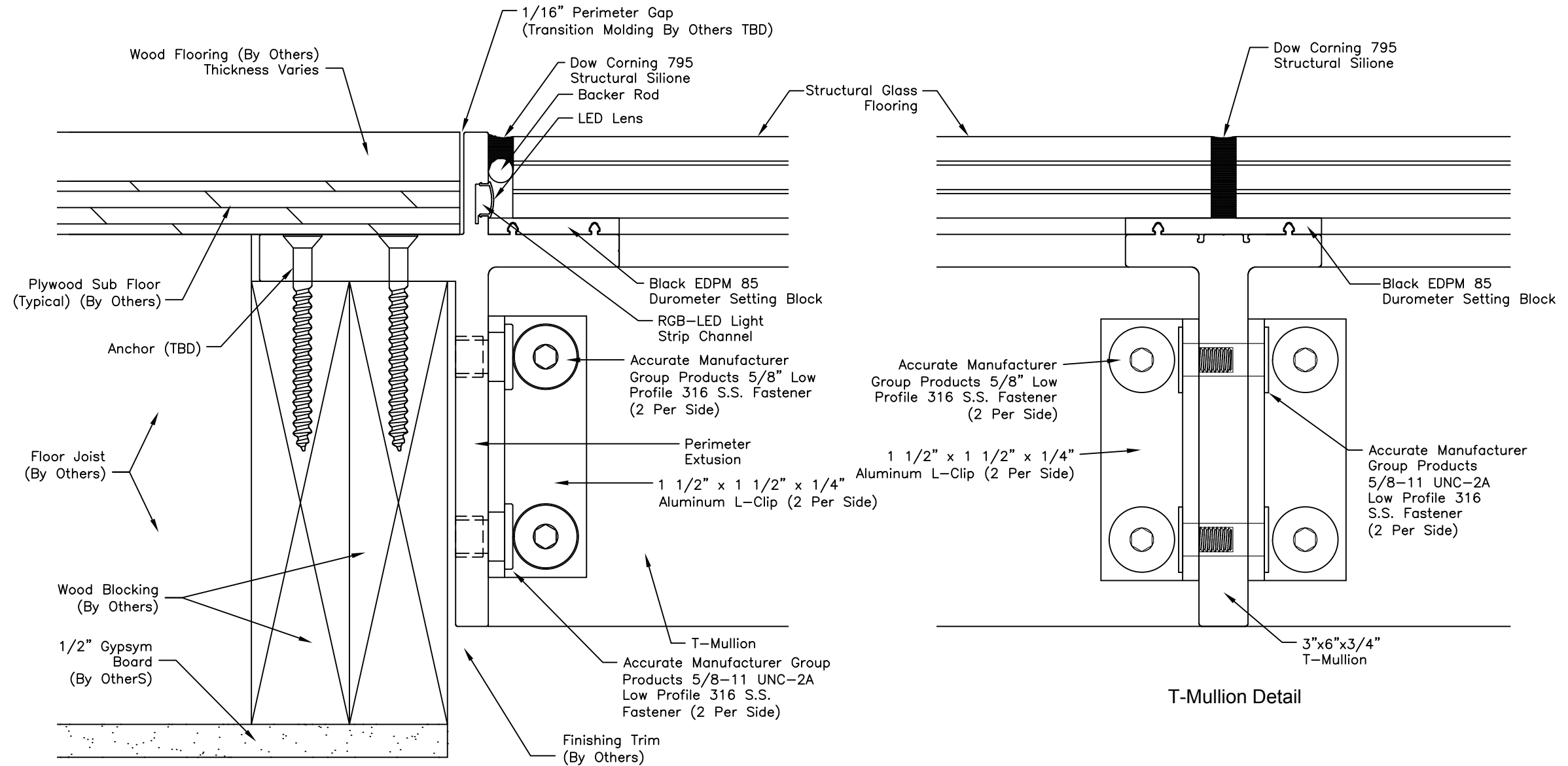
Interior Wood Floor Detail W/T-Mullion
