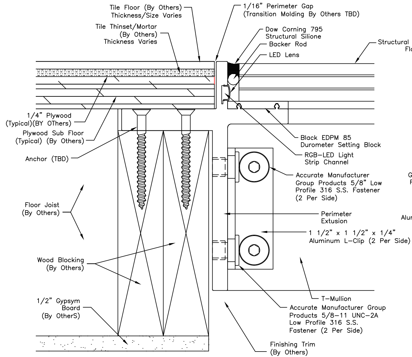
Interior Tile Flooring Detail W/T-Mullion
