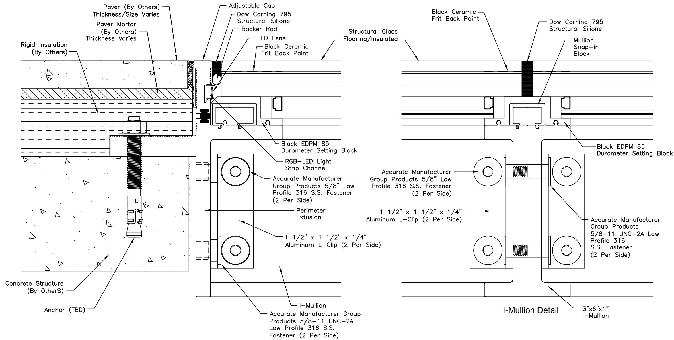
Exterior Recessed Paver Detail W/I-Mullion
